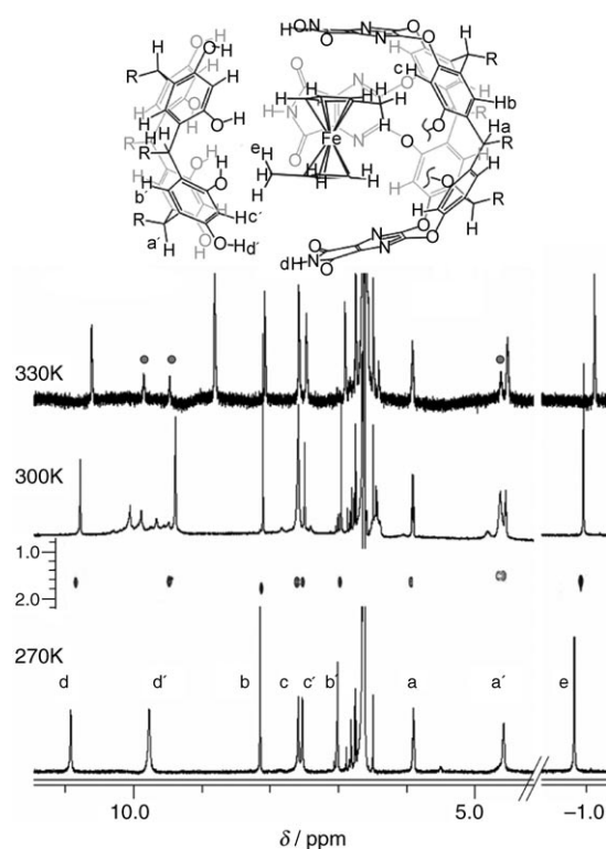
Figure 6. Partial ^1\text{H} NMR spectra ( [\text{D}_{12}]\text{mesitylene} , 600 MHz) of dimethylferrocene ( 11 ; 20 mM) mixed with 4 (4 mM) and 2 (2 mM) at various temperatures. Some of the peaks for hexamer 1 are marked with gray circles (●) in the spectrum obtained at 330 K. The DOSY spectrum ( [\text{D}_{12}]\text{mesitylene} , T = 300\text{ K} , 400 MHz) of 11 in 6 is included below the spectrum obtained at 300 K.
